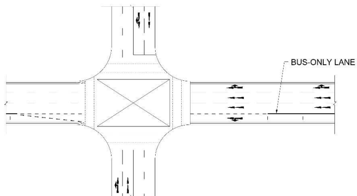
AT SIGNALISED INTERSECTION FOR BUS-ONLY LANE
